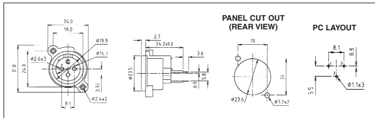
XNACF4V - 3 Pin vertical PCB mounting Female XLR with latch. Gold plated PbRz contacts standard.
