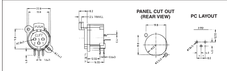
XNACF3 - 3 Pin right angle PCB mounting Female XLR with latch. Nickel Silver or Gold plated PbRz contacts available.
