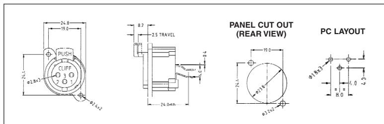
XNACF3V - 3 Pin vertical PCB mounting Female XLR with latch. Nickel Silver or Gold plated PbRz contacts available.
