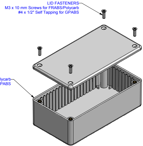
EXPLODED VIEW OF ENCLOSURE
