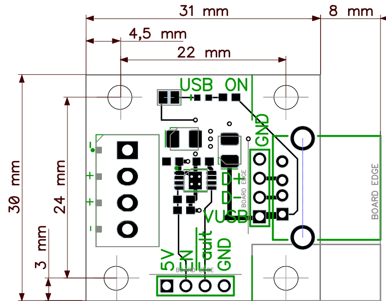
PCB angle bracket RICHCO PCB-MB-1
