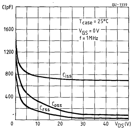
Capacitance variation
