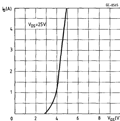
Transfer characteristics
