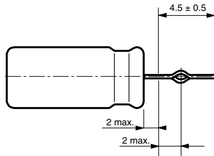
5 ≤ Ø D ≤ Leads bent open, shortened and formed EKS 09... (S = 5 mm)
