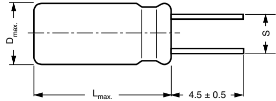
10 ≤ Ø D ≤ 18 Leads shortened and formed EKS 06... (S = 5 / 7.5 mm)
