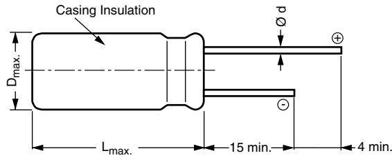
5 ≤ Ø D ≤ 18 Long leads EKS 00...
