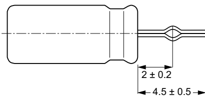
5 ≤ Ø D ≤ 18 Shortened leads EKS 05... (S = 2 / 2.5 / 3.5 / 5 / 7.5 mm)
