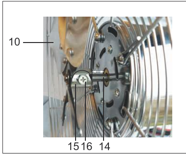
Fig.3: Montage Rotor
