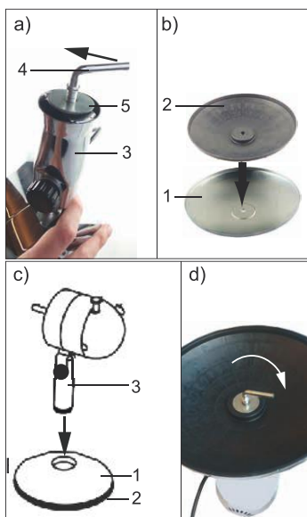
Fig. 136: Montage Basis
