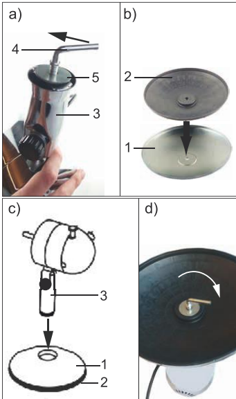
Fig.51: Montage basis
